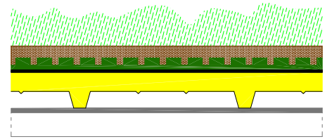
part. tetto verde green roof
